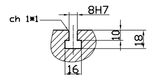
slots detail (scale 1.5)
